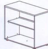
OPEN SHELF CABINET EXO 880 804W x 402D x 848H
