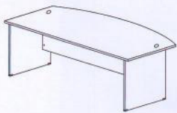
EXECUTIVE TABLE EXT 180A 1800W x 900D x 750H
