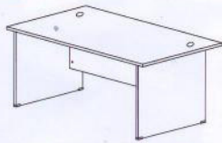
STANDARD TABLE EXT 188 1800W x 800D x 750H EXT 187 1800W x 700D x 750H EXT 157 1500W x 700D x 750H EXT 127 1200W x 700D x 750H
