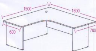
SUPERIOR COMPACT TABLE (L) EXL 552 1500W x 1500D x 600 x 600 x 750H EXL 1515 1500W x 1500D x 700 x 600 x 750H EXL 1815 1800W x 1500D x 700 x 600 x 750H
