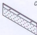
SOLID PANEL W/O RACEWAY C/W HANGING RAIL AT BOTTOM 18 SP/WR2 1800W x 450H x 18THK 1800W x 600H x 18THK 1500W x 450H x 18THK 1500W x 600H x 18THK 1200W x 450H x 18THK 1200W x 600H x 18THK
