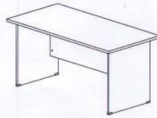
STANDARD TABLE EXT 126 1200W x 600D x 750H
