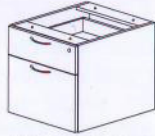
FIXED PEDESTAL 2D QH 2 400W x 470D x 480H
